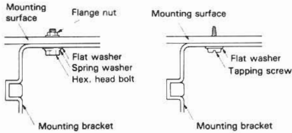
Fig. c Mounting bracket installation
